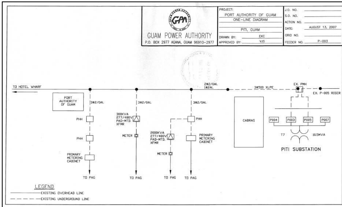
Figure 2.4-1 GPA Power Supply Schematic for PAG
