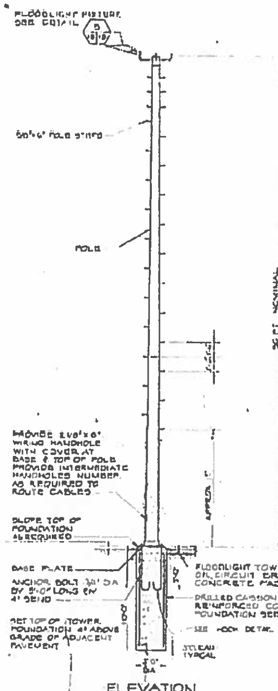
ELEVATION FLOODLIGHT TOWER POLE DETAIL NO SCALE
